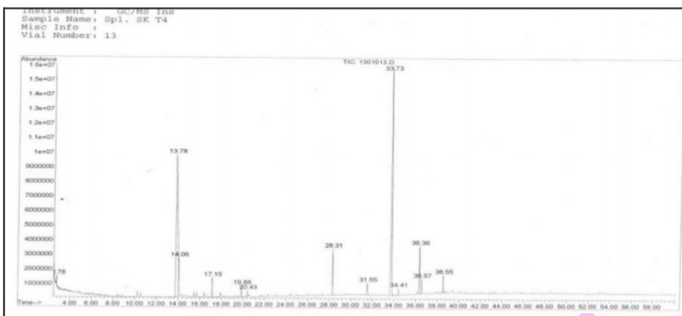
2 Figure 5. Graphic of compounds that are contained in coconut fibers liquid smoke at pyrolysis temperature of 400 \pm 10^\circ\text{C} detected by GC MS
