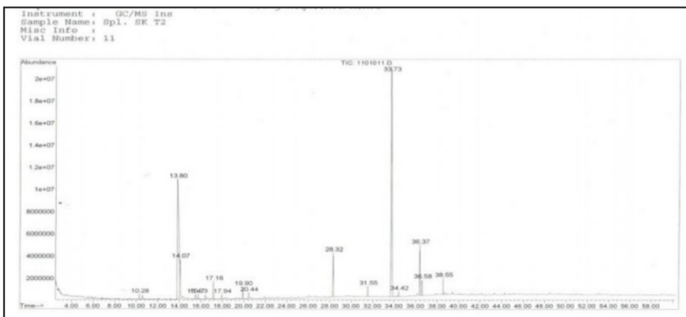
Figure 3. Graphic of compounds that are contained in coconut fibers liquid smoke at pyrolysis temperature of 200 \pm 10^\circ\text{C} detected by GC MS
