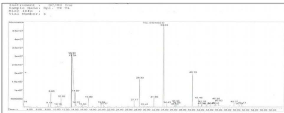
7 Figure 9. Graphic of compounds that are contained in coconut shell liquid smoke at pyrolysis temperature of 400 \pm 10^\circ\text{C} detected by GC MS
