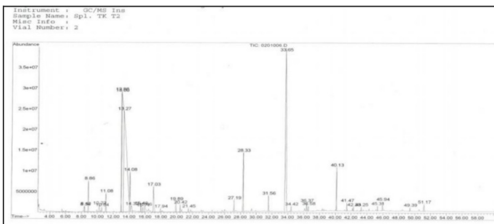
7 Figure 7. Graphic of compounds that are contained in coconut shell liquid smoke at pyrolysis temperature of 200 \pm 10^\circ\text{C} detected by GC MS
