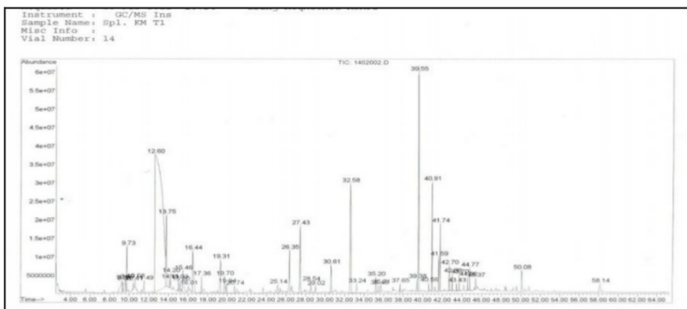
3 Figure 10. Graphic of compounds that are contained in cinnamon liquid smoke at pyrolysis temperature of 100 \pm 10^\circ\text{C} detected by GC MS
