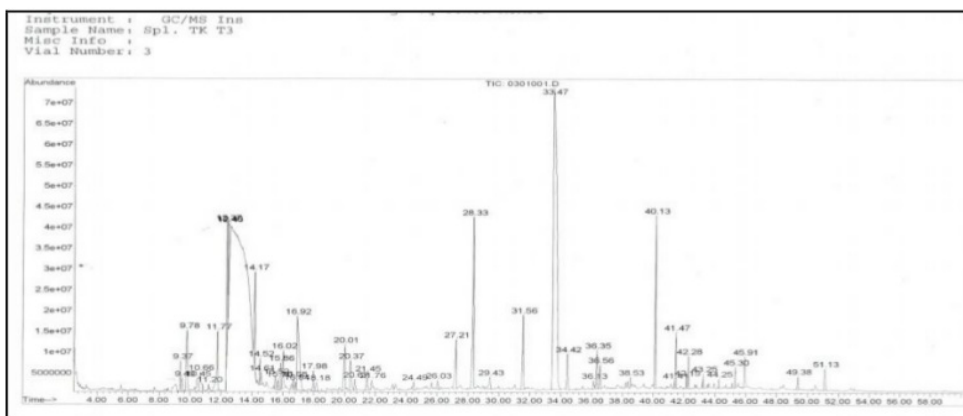
7 Figure 8. Graphic of compounds that are contained in coconut shell liquid smoke at pyrolysis temperature of 300 \pm 10^\circ\text{C} detected by GC MS
