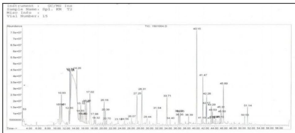
3 Figure 11. Graphic of compounds that are contained in cinnamon liquid smoke at pyrolysis temperature of 200 \pm 10^\circ\text{C} detected by GC MS
