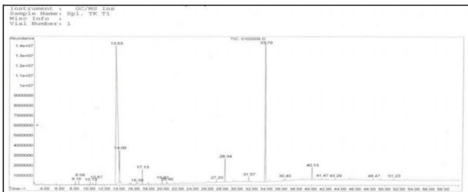
7 Figure 6. Graphic of compounds that are contained in coconut shell liquid smoke at pyrolysis temperature of 100 \pm 10^\circ\text{C} detected by GC MS
