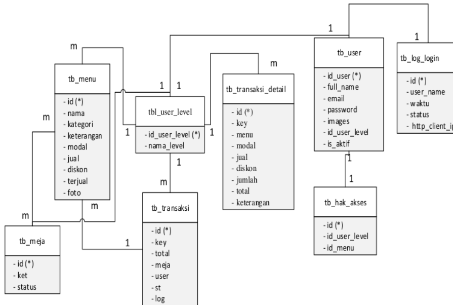
Gambar 5. Entity Relational Diagram
