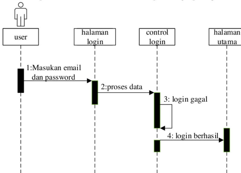
Gambar 1. Sequence Diagram Proses Login
