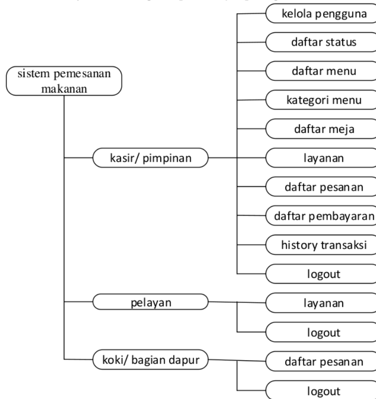
Gambar 6. Sitemap Desain Interface
