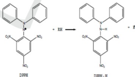
Figure 2: DPPH radical reduction reaction by antioxidants.
