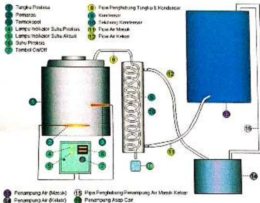
Figure 3 . Equipment make of liquid smoke
