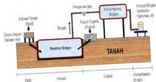
Figure 1. Household scale biogas digesters
