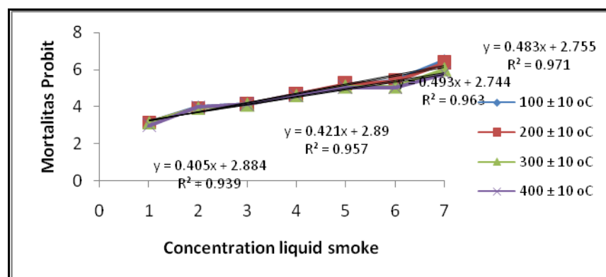
Figure 4. Mean mortality Probit value of Multiple Temperature Level Pyrolysis with different concentrations of liquid smoke
