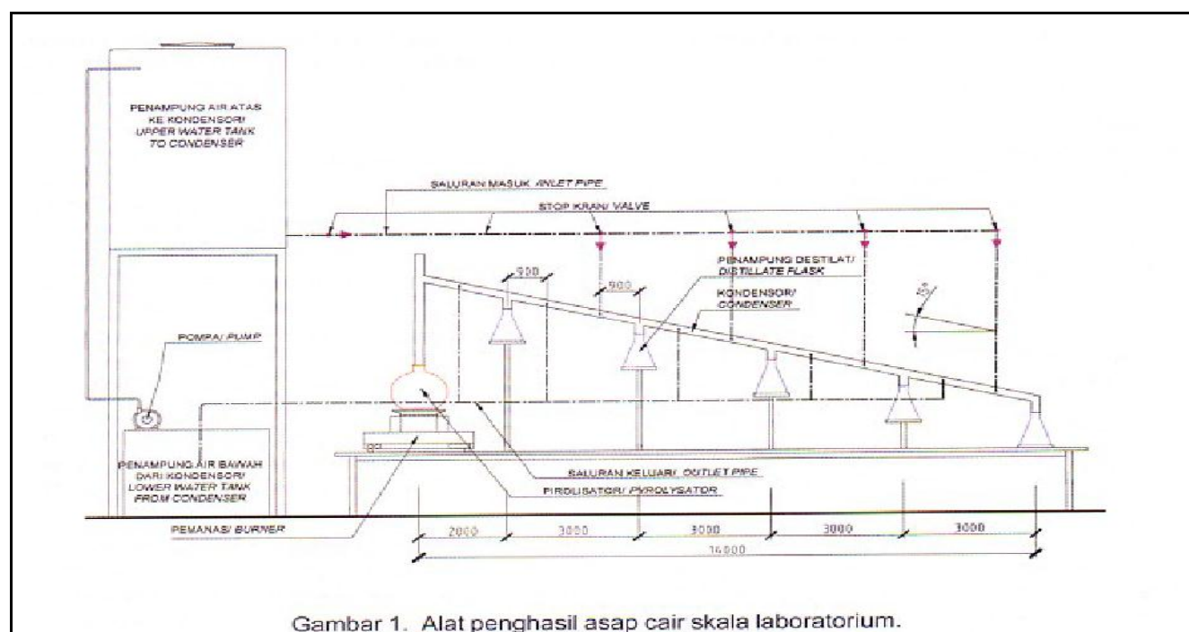
Figure 1.Liquid smoke device of a laboratory scale
